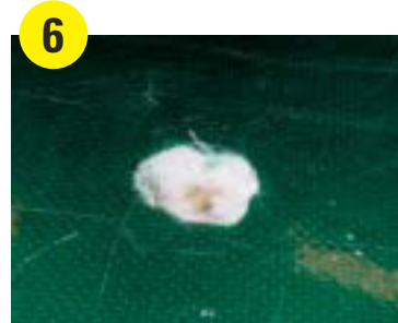
6 After the damaged fiberglass is removed, make sure the foam core is perfectly dry. Remove damaged or crushed foam.
