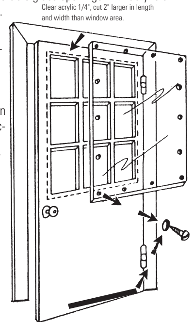
Round-head screws 1/2" in length with finishing washers.
